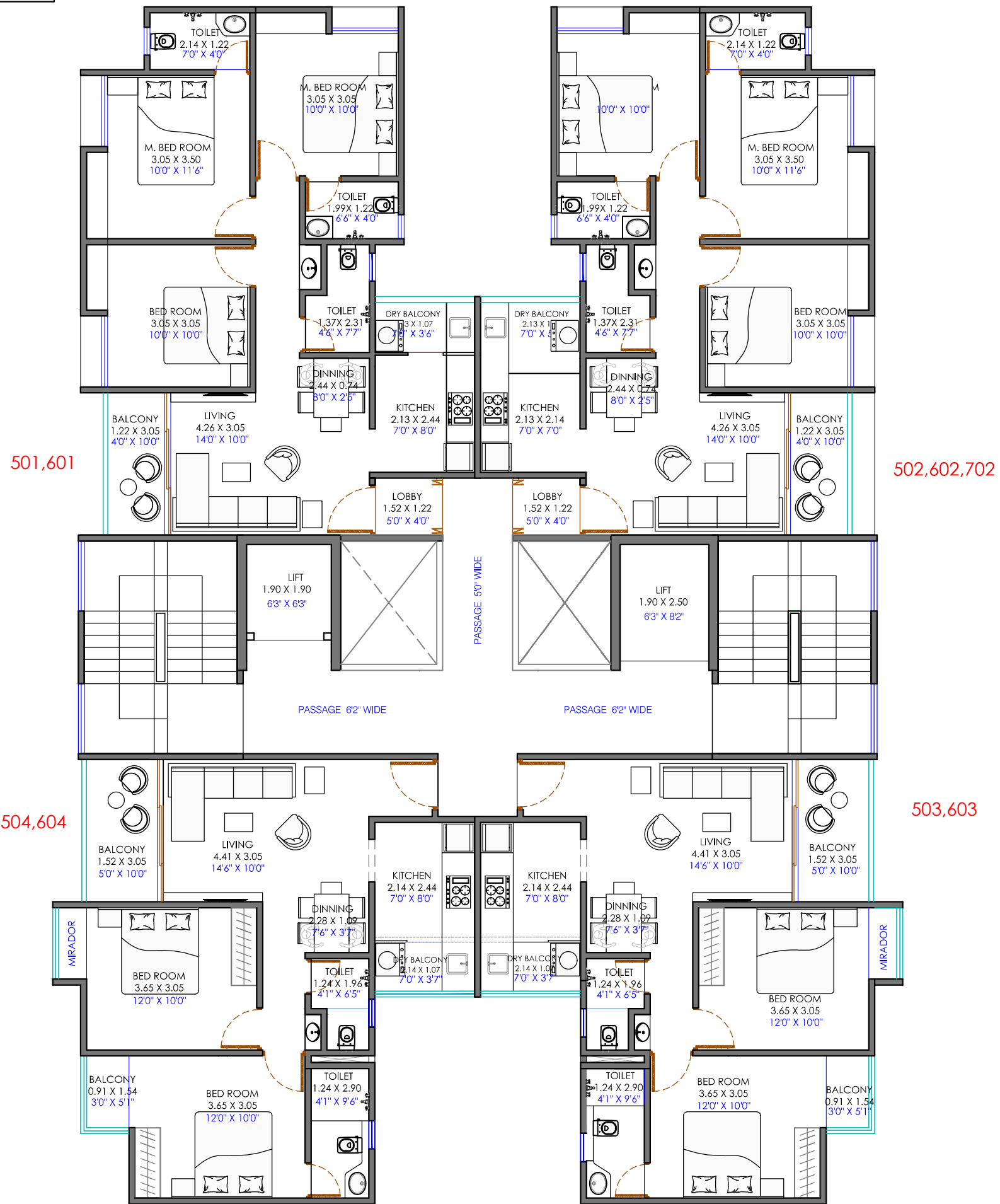
TYPICAL - 5TH,6TH,7TH,FLOOR PLAN
