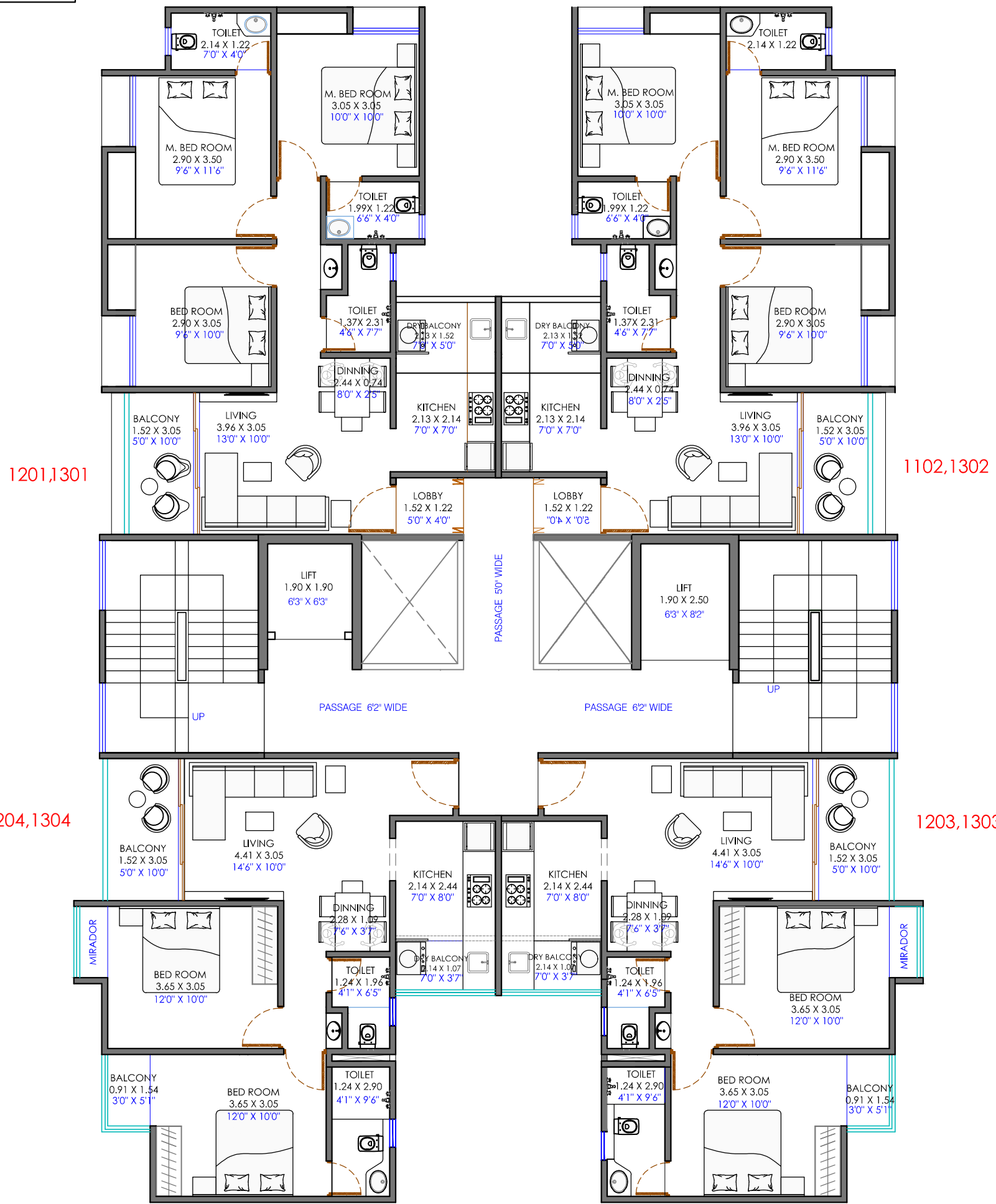
TYPICAL 11,12,13 TH. FLOOR PLAN
