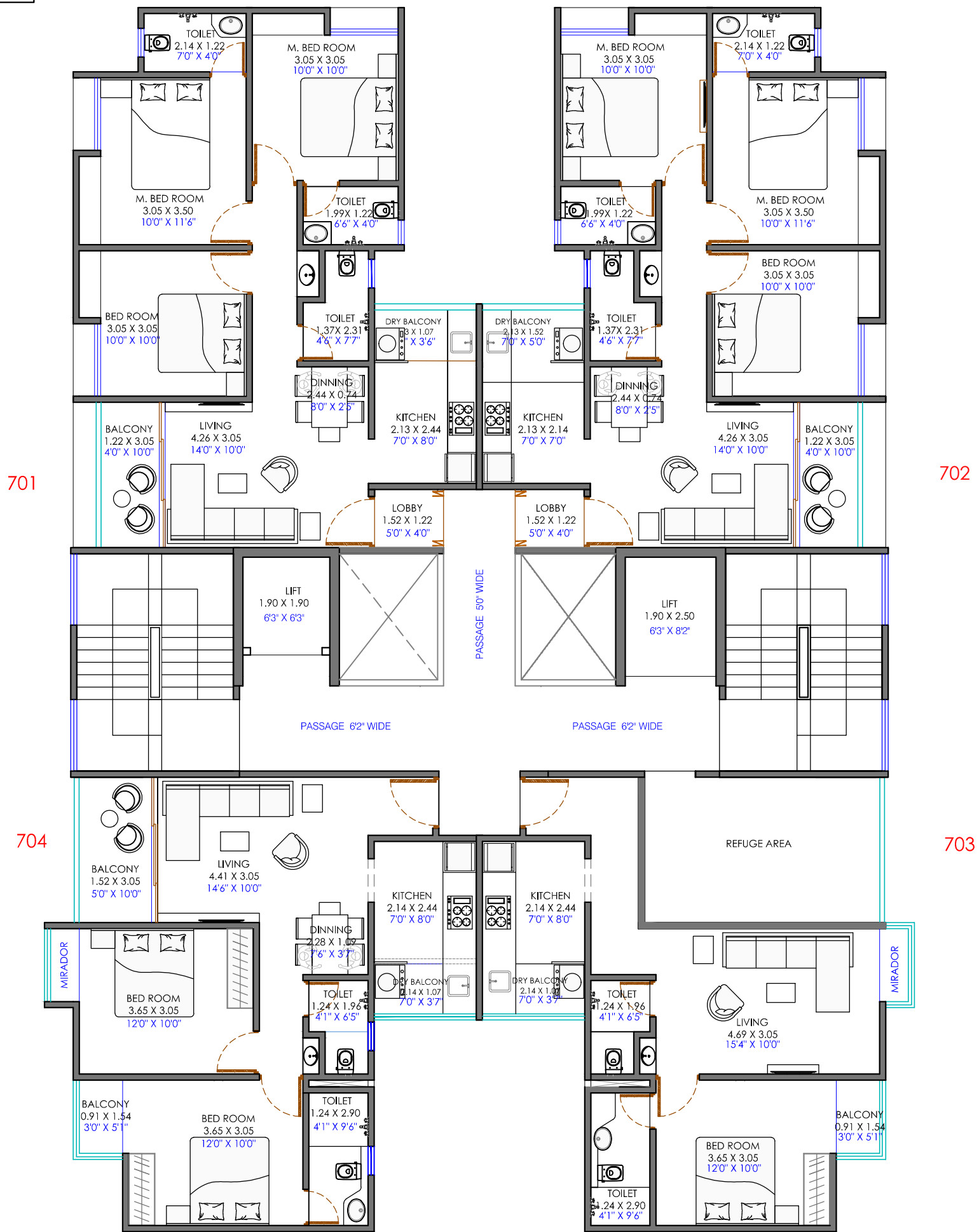
TYPICAL - 7TH,11TH FLOOR PLAN
